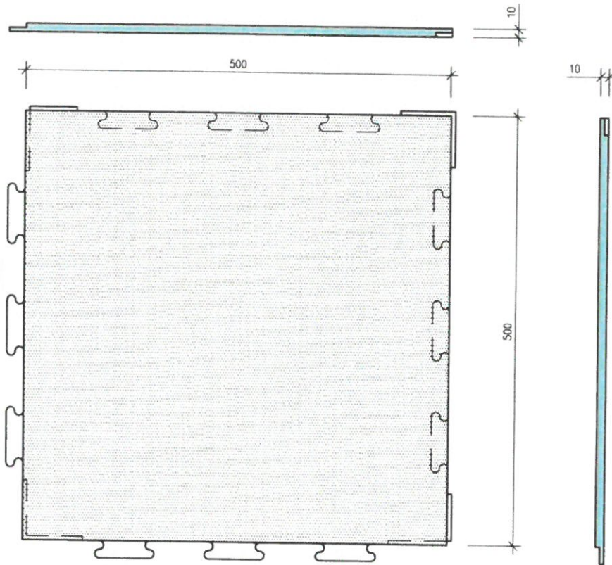
Detail "plus"- Verriegelung
